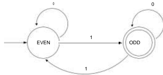
Gambar 1. Contoh Soal Graph FSA
