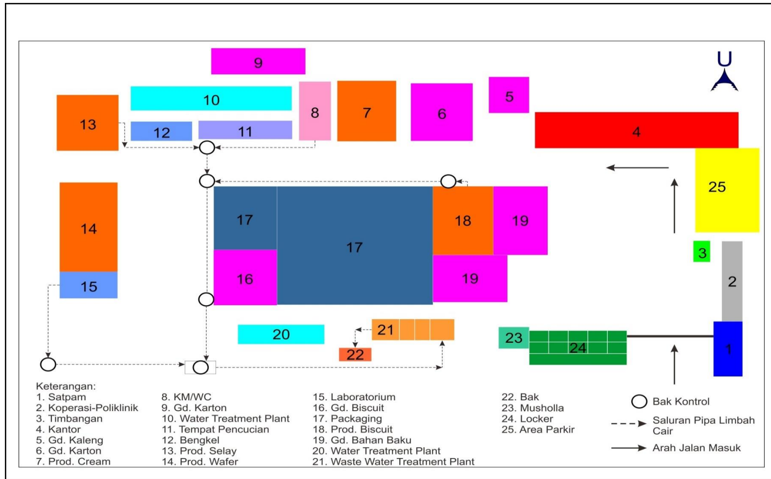
Gambar I.2 Layout PT Interbis Sejahtera Food Industry
